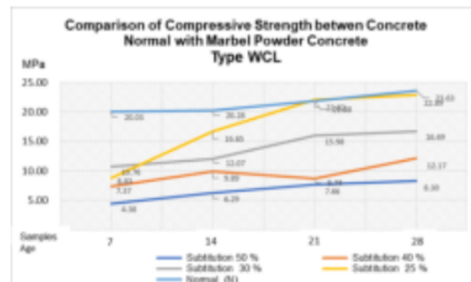
Figure-10. Comparison of the WCL type pressure test results on all types substitution of Graphite Carbon marble powder.
