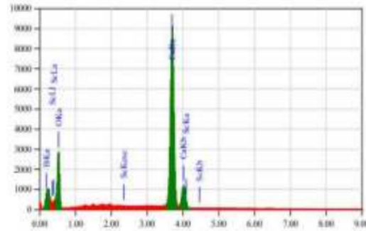
Figure-4. EDS results marble powder.
