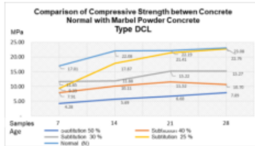
Figure-8. Comparison of the DCL type pressure test results on all types substitution of graphite carbon marble powder.
