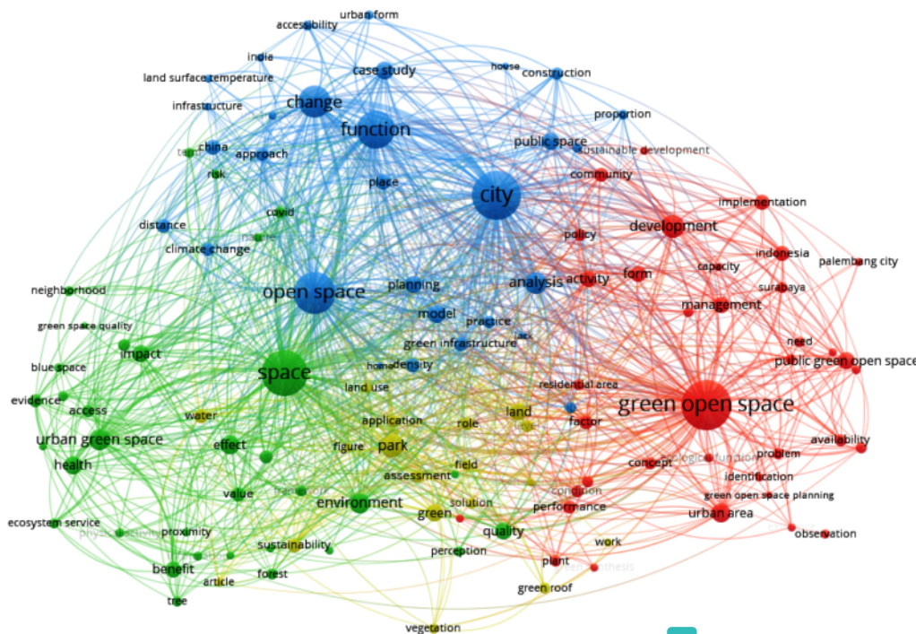
Fig. 1. Grouping of green open space study themes. (Source: Vosviewer analysis results and publish or perish). (For interpretation of the references to color in this figure legend, the reader is referred to the Web version of this article.)
