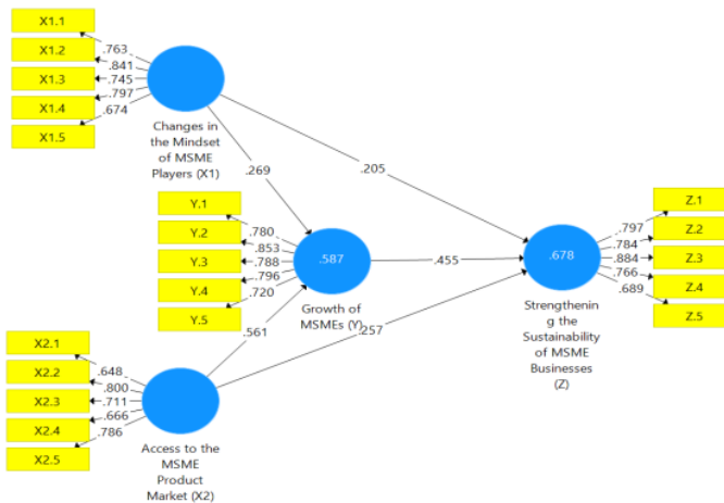
Fig.3: PLS Algorithm model 1
