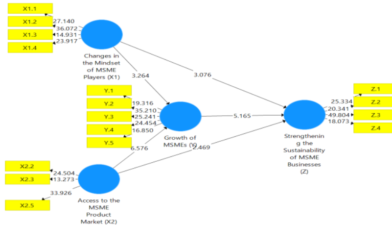
Fig.5: Bootstrapping test Source: Author's findings, 2024.
