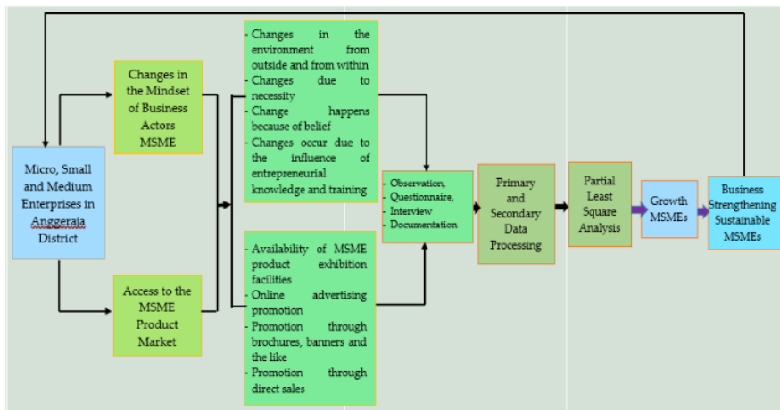
Fig.2: Model SEM PLS. Source: Author's findings, 2024.
