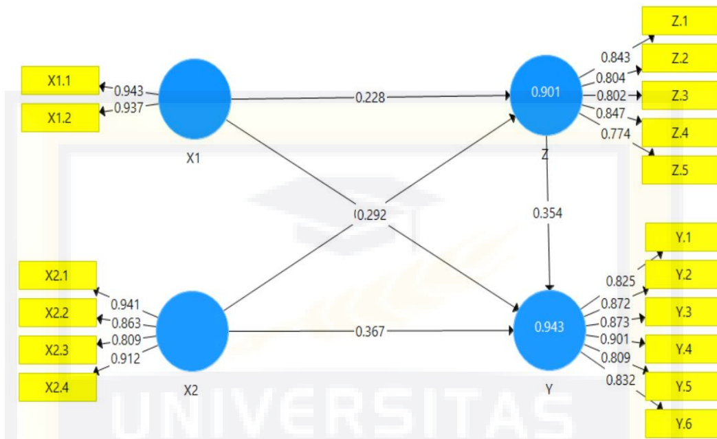
Gambar 4.1. PLS Algorithm
