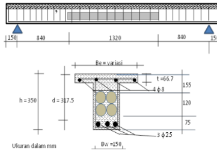
Gambar 8. Dimensi Balok T beton bertulang berlapis
