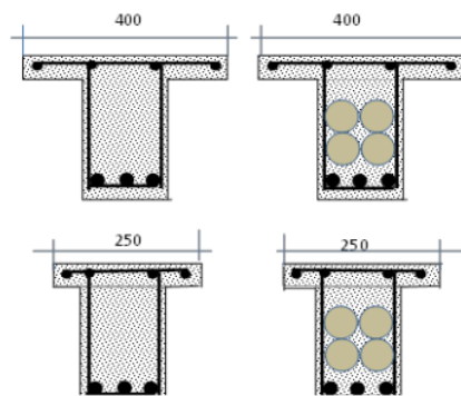
Gambar 8. Variasi Balok T beton bertulang berlapis
