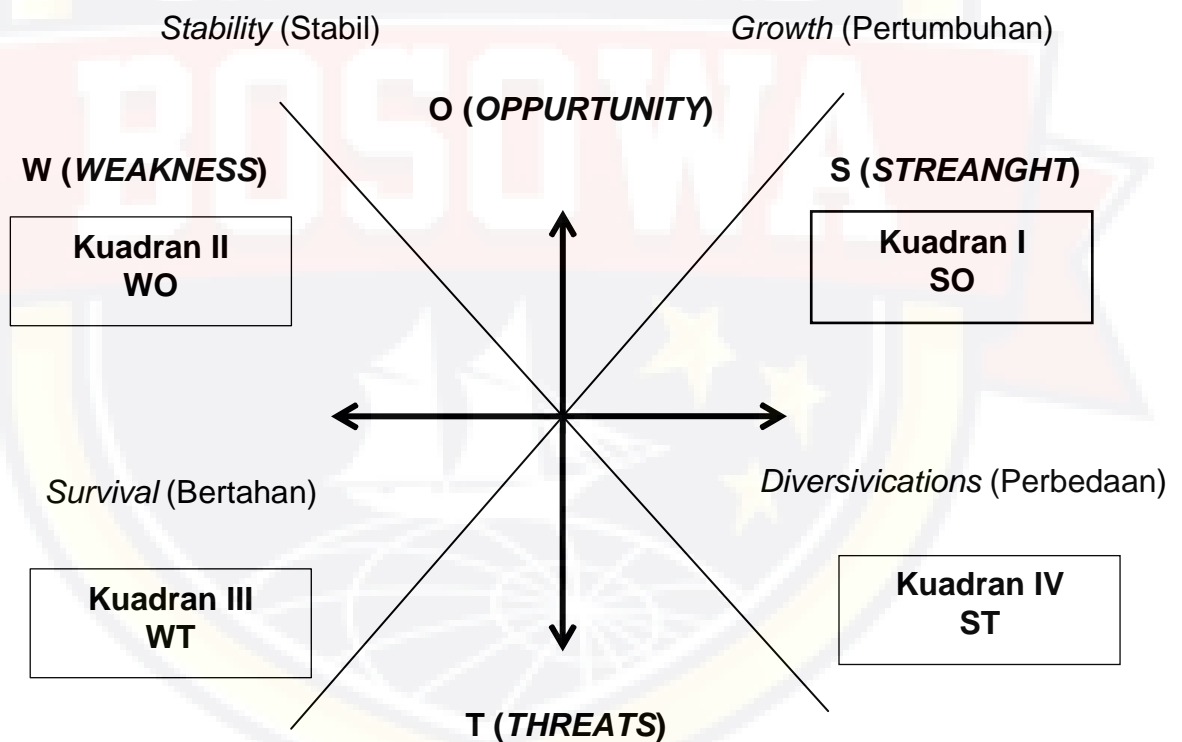
Gambar 3.1 Diagram Penentuan Strategi Prioritas Analisis SWOT
