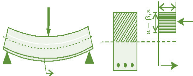
Fig. 1 Flexural action of reinforced concrete beam
