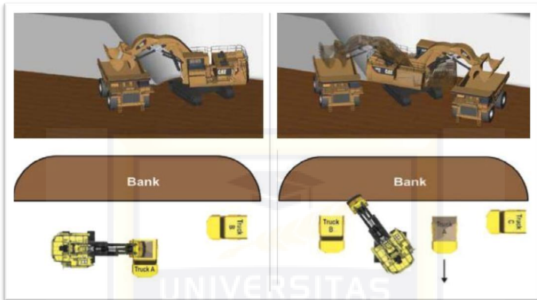
Gambar 2.9 Single Side dan Double Side Loading (Caterpillar 2015)
